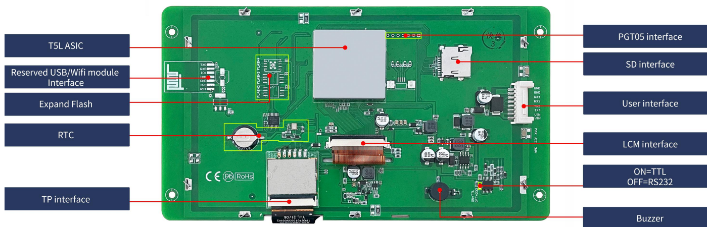
Hardware interface
