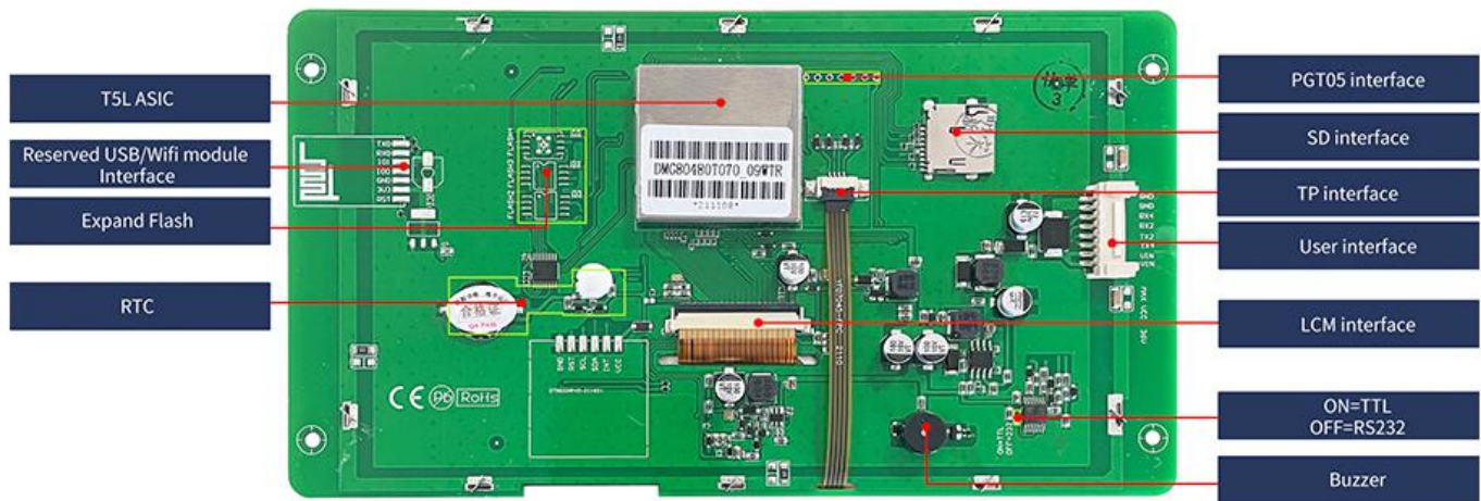
Hardware interface
